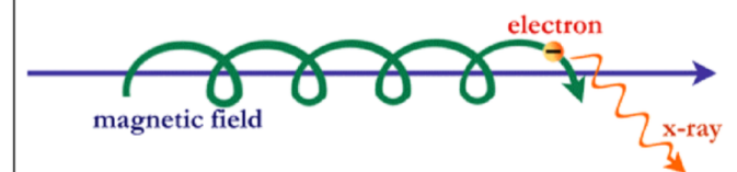
Synchrotron Radiation
