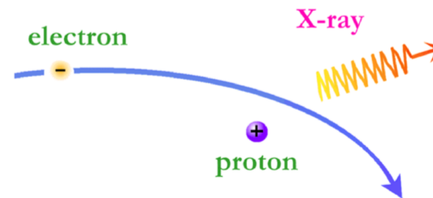
X-ray Producing Collision
