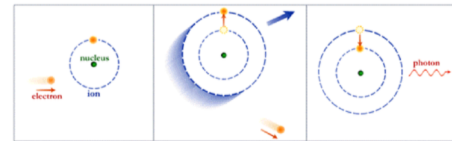
Atomic Emission
